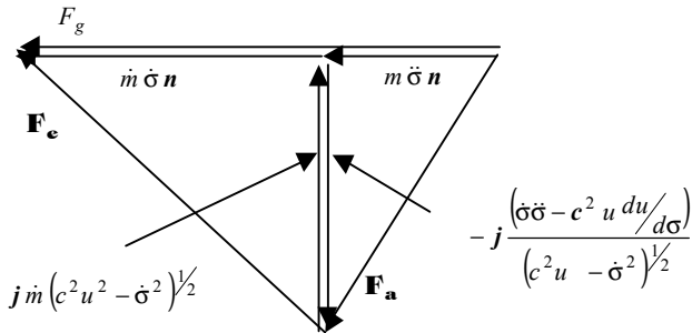
Fig. 2.2 – Balanced Force Vector Diagram for Rectilinear Gravitational Motion.
