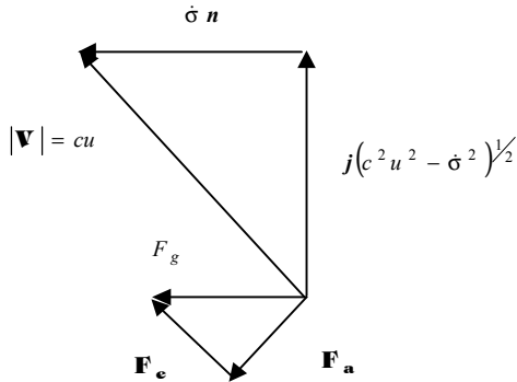
Fig. 2.1 – Components of F_g with Respect to \mathbf{V} .
